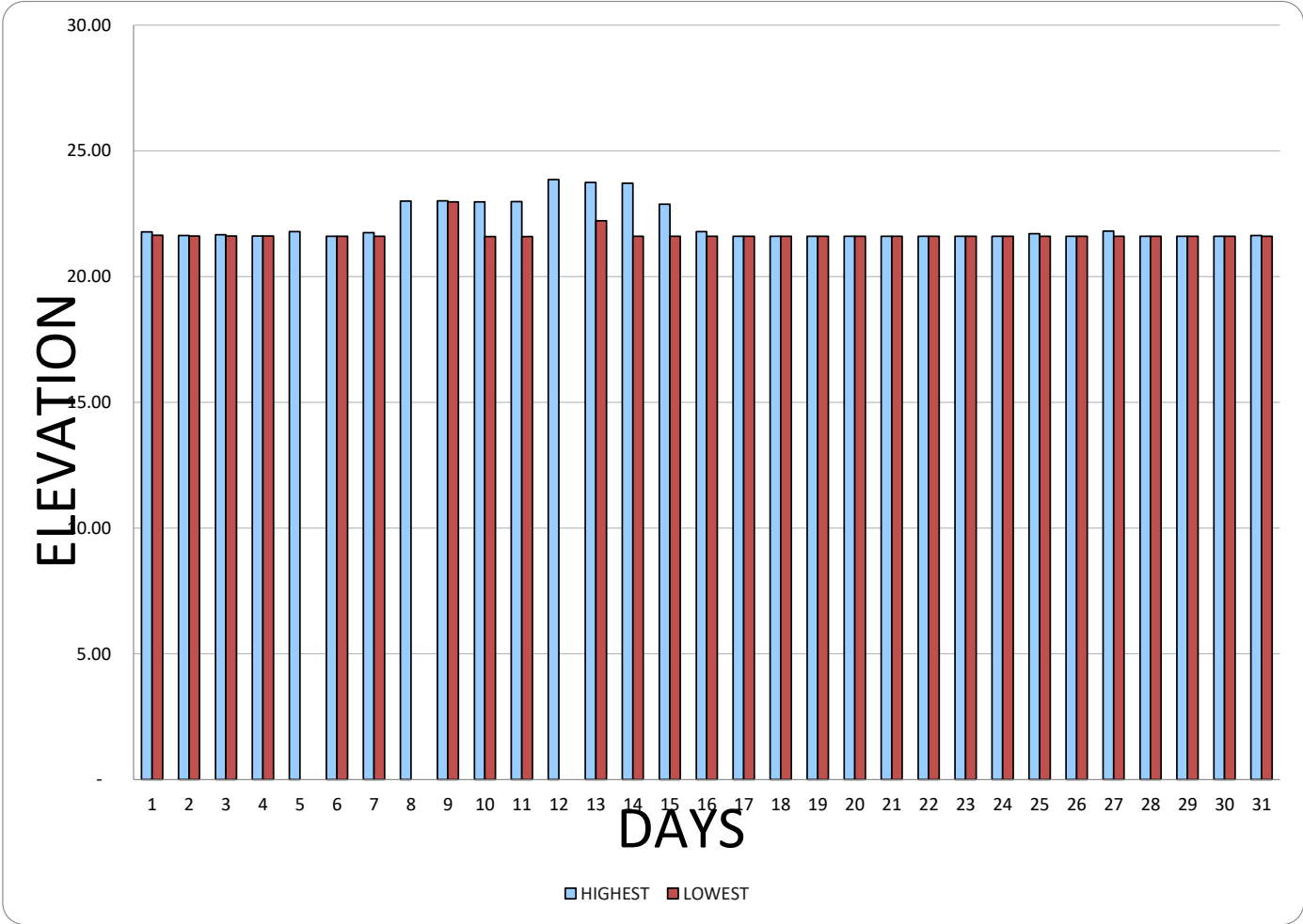
RECORDED DAILY HIGHEST AND LOWEST WATER ELEVATION MONTALBAN WATER LEVEL GAUGING STATION March 1-31, 2024
